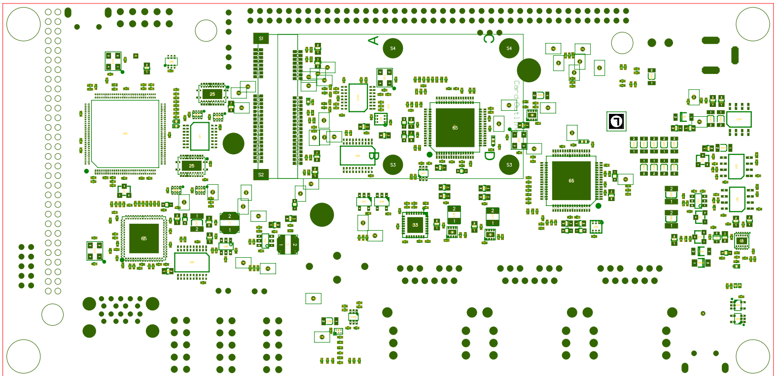
Component Placement Diagram: Bottom Side 1566.1 (PBA-C-25)
