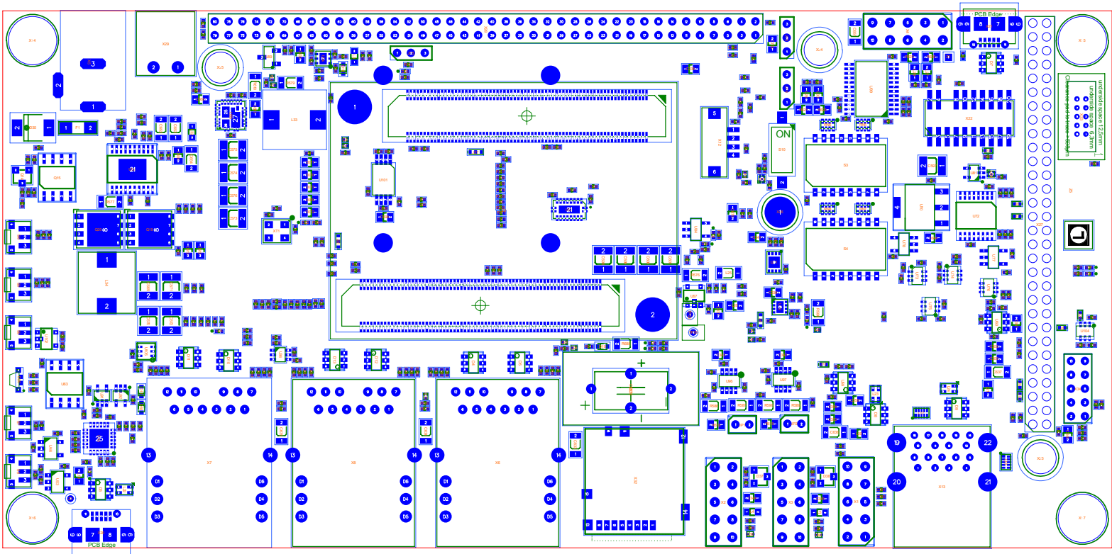
Component Placement Diagram: Top Side 1566.1 (PBA-C-25)
