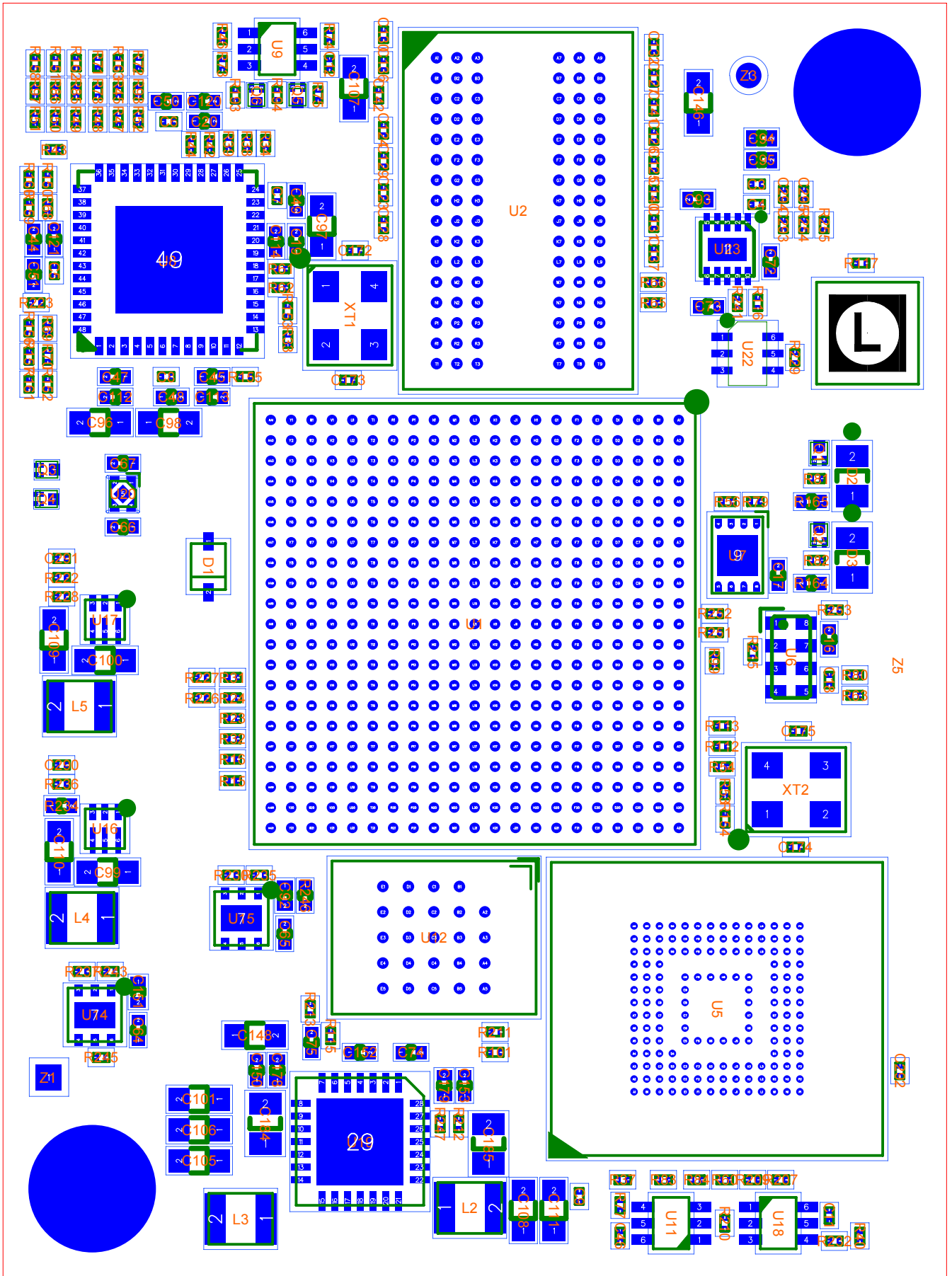
Component Placement Diagram: Top Side 1565.1 (PCM-072)
