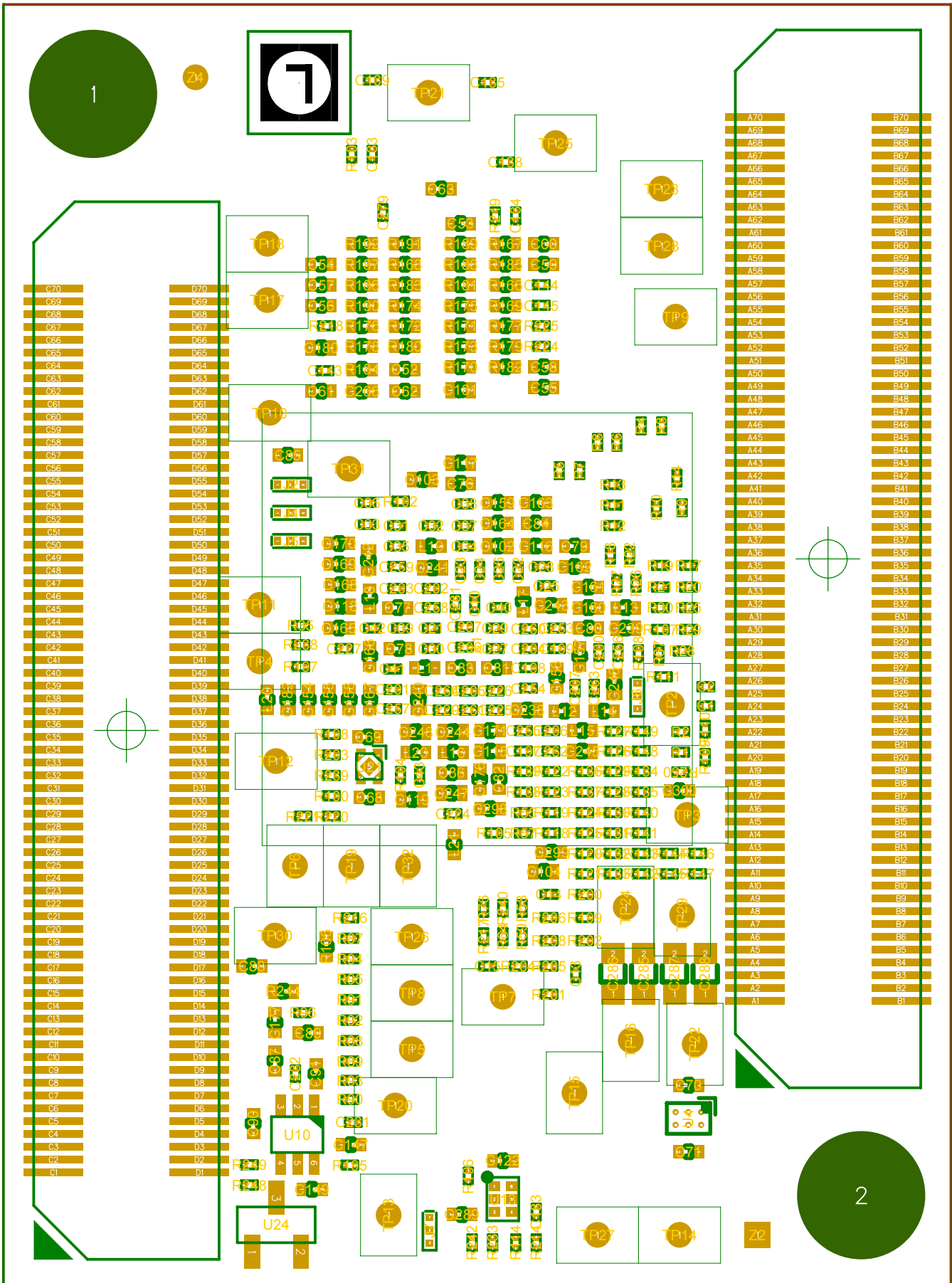
Component Placement Diagram: Bottom Side 1565.1 (PCM-072)
